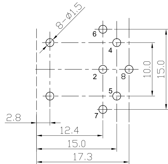
P.C.B LAYOUT BOTTOM VIEW
